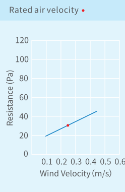
Resistance-Wind Velocity Graph
