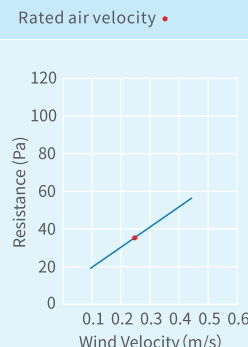
Resistance-Wind Velocity Graph
